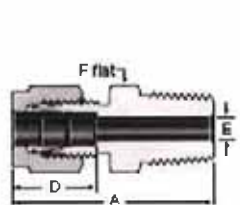
ISO/BSP Tapered Thread (RT)
